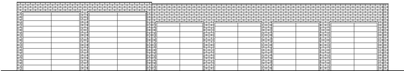
Existing North West Elevation scale A3 1:100
