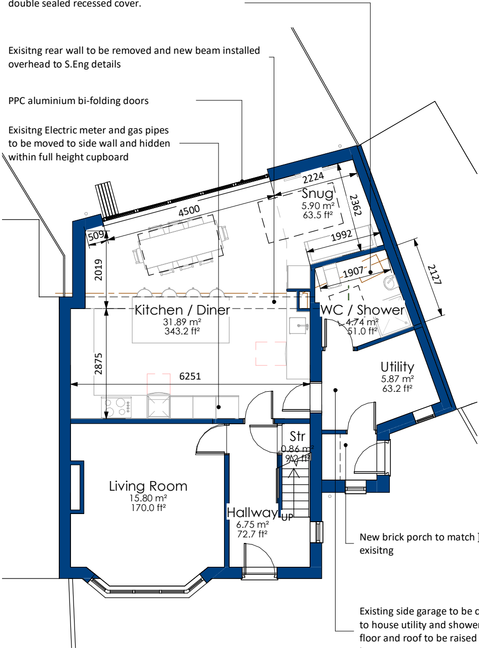
Ground Floor Plan As Proposed 1 : 100
