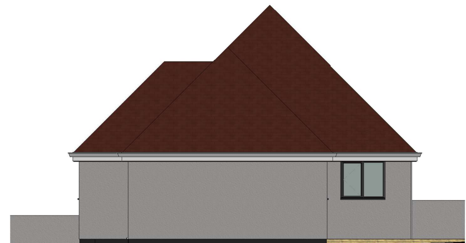
4 West Elevation 1 : 100
