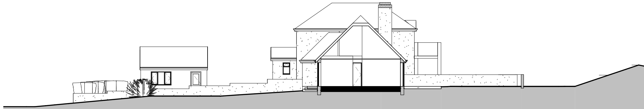
1 North South Site Section 1 : 200
