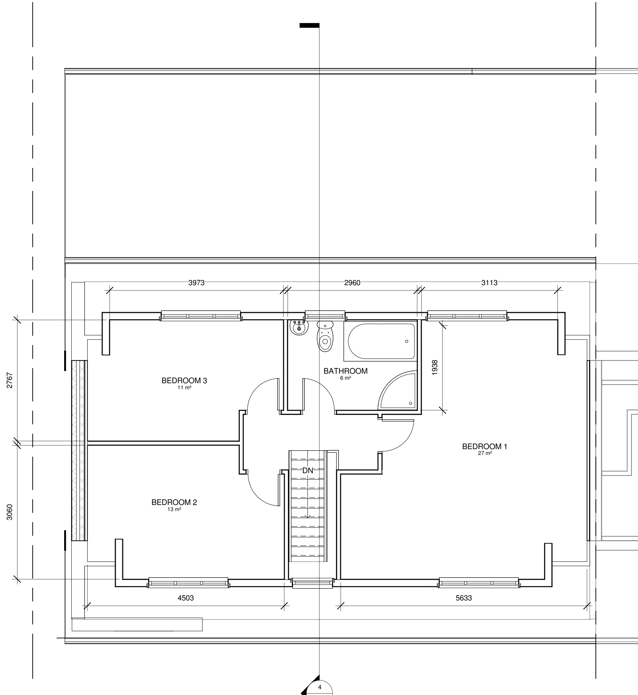
2 1 - Proposed First Floor 1 : 50
