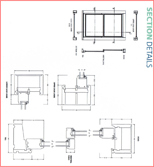
Frame Details
