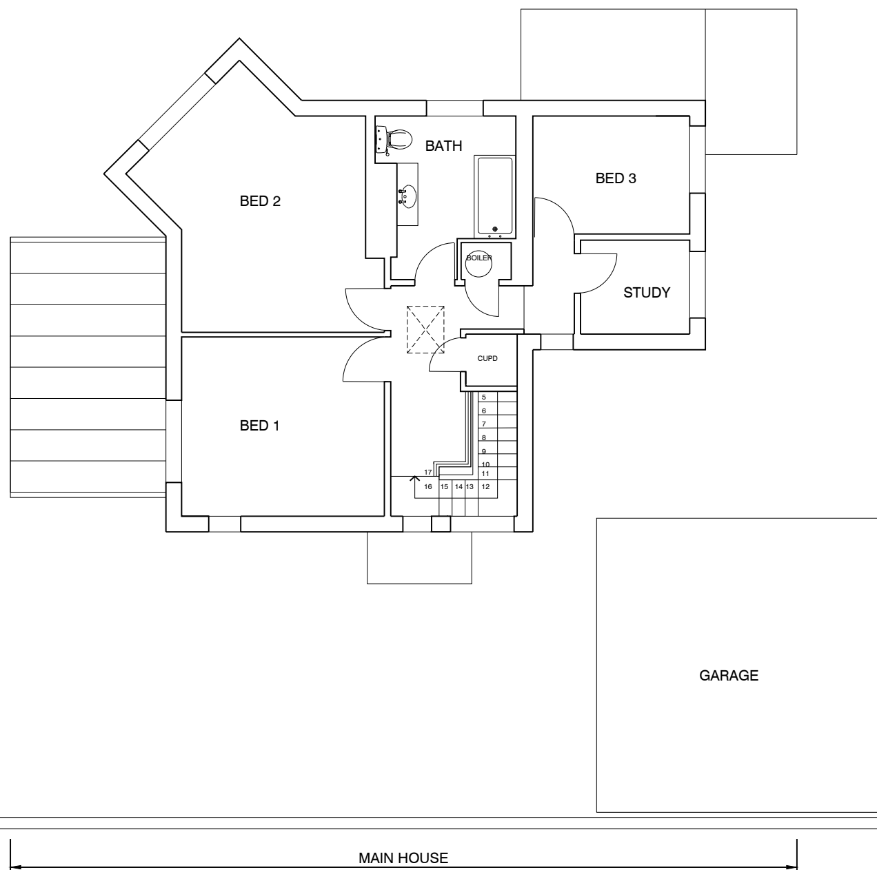
EXISTING FIRST FLOOR PLAN - MAIN HOUSE SCALE 1:100 @ a3
