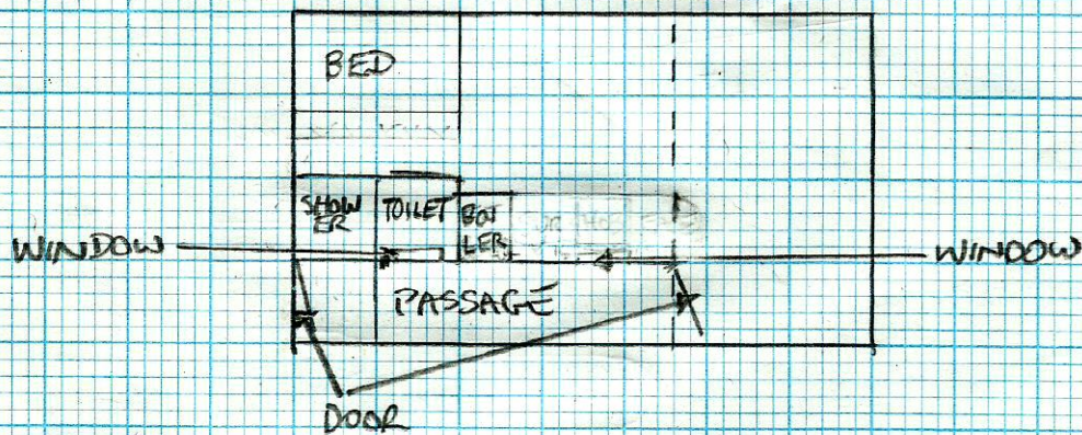
FLOOR PLAN
