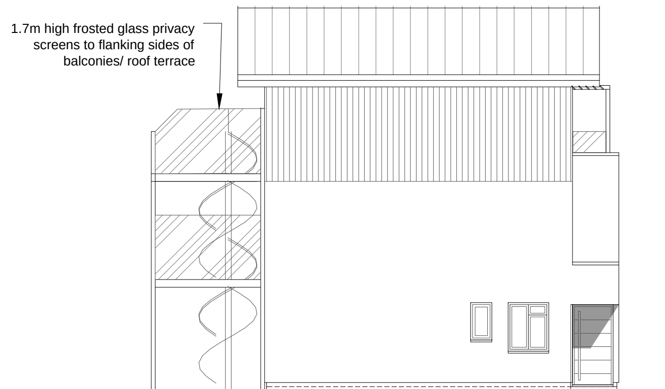
SIDE (NE)
