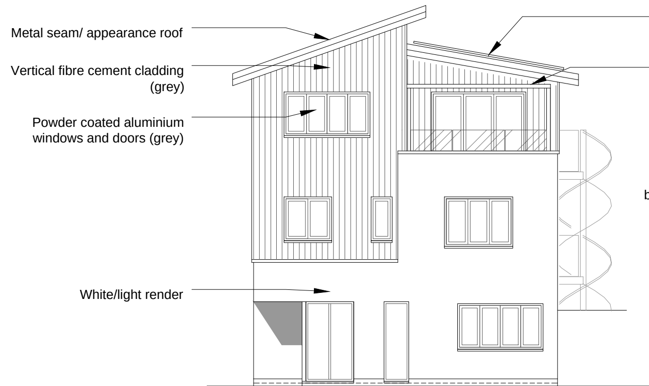
FRONT (NW)
