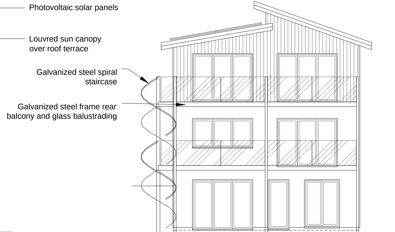
REAR (SE)
