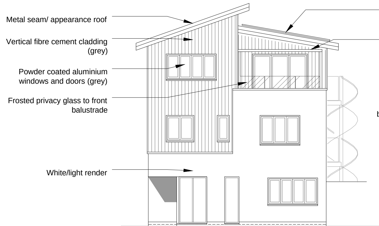
FRONT (NW)
