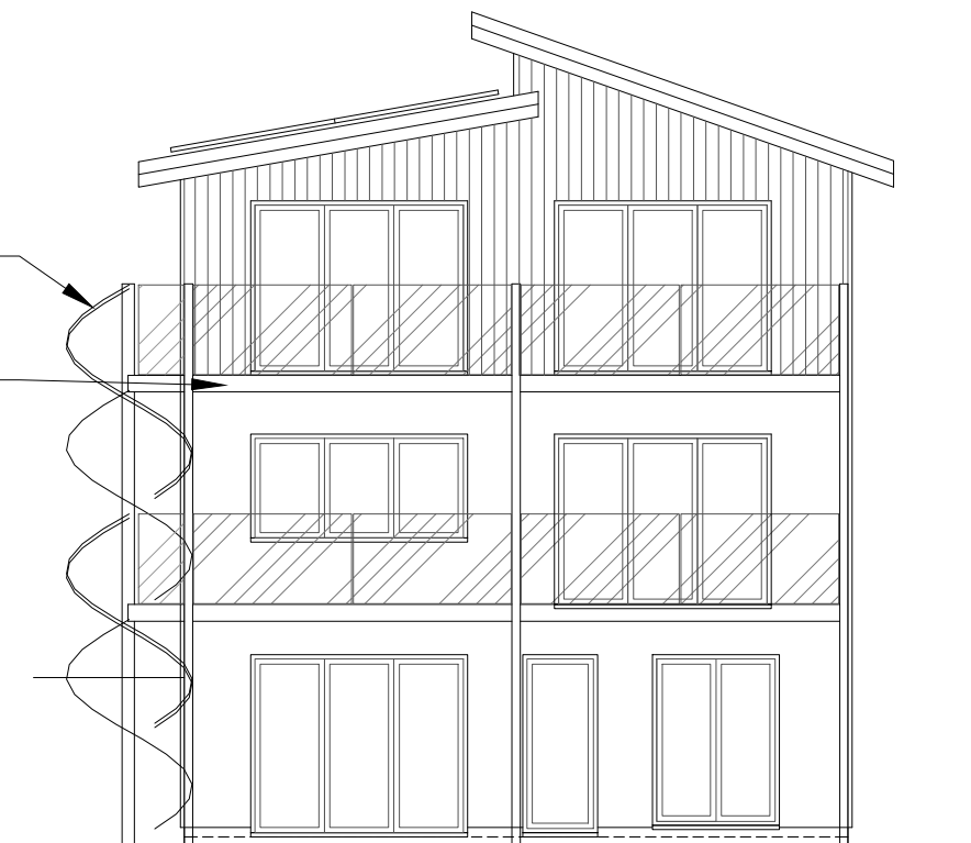
REAR (SE)
