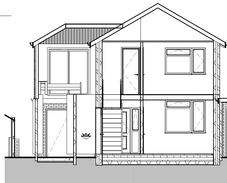
1 North South Site Section 1 : 100
