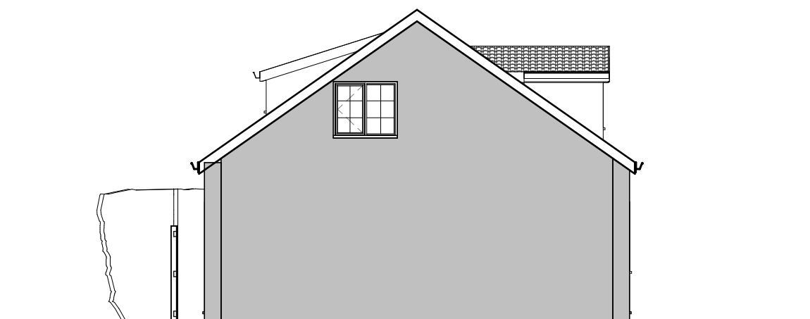
3 South Elevation 1 : 100
