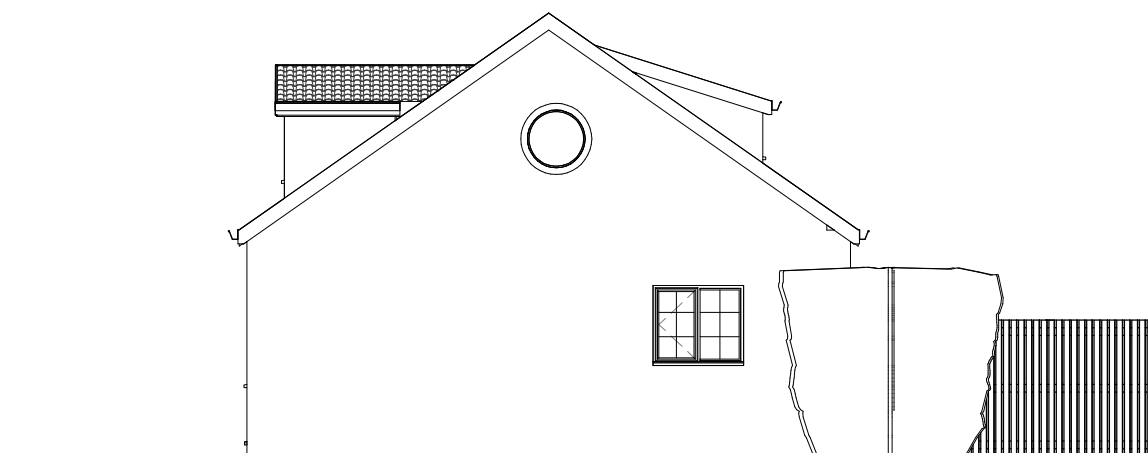
2 North Elevation 1 : 100
