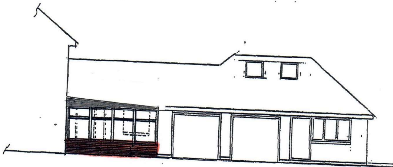
SOUTH ELEVATION.
