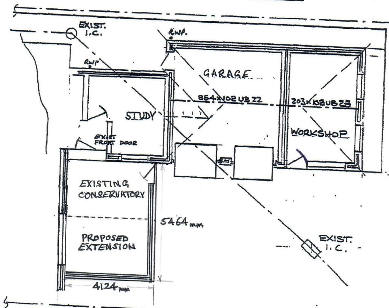
PROPOSED SITE PLAN [SCALE 1:100]
