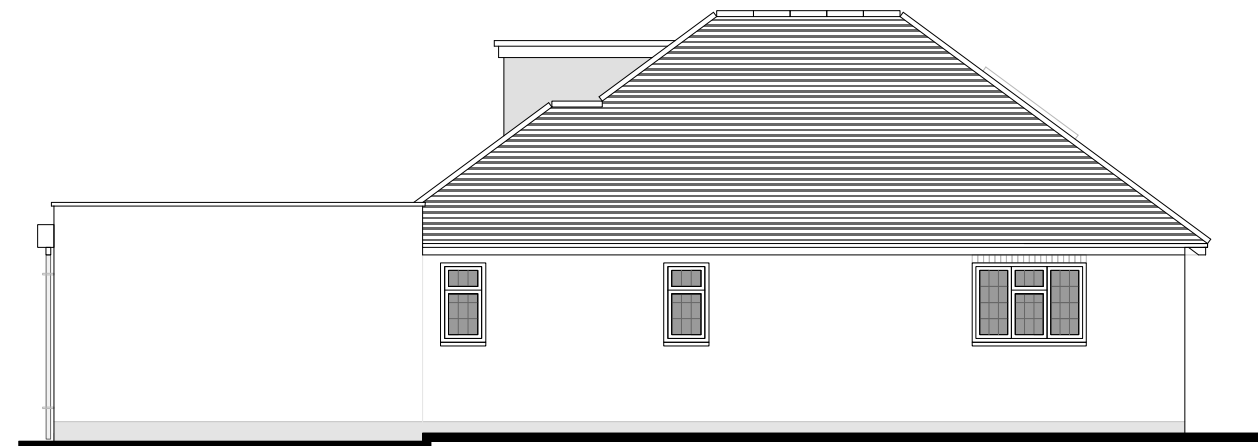
Proposed Side Elevation at 1:100 scale NORTH EAST
