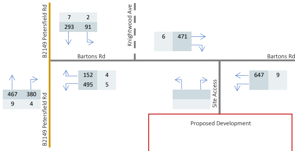
2018 Recorded Traffic Flows - PM Peak Hour (17:00-18:00)
