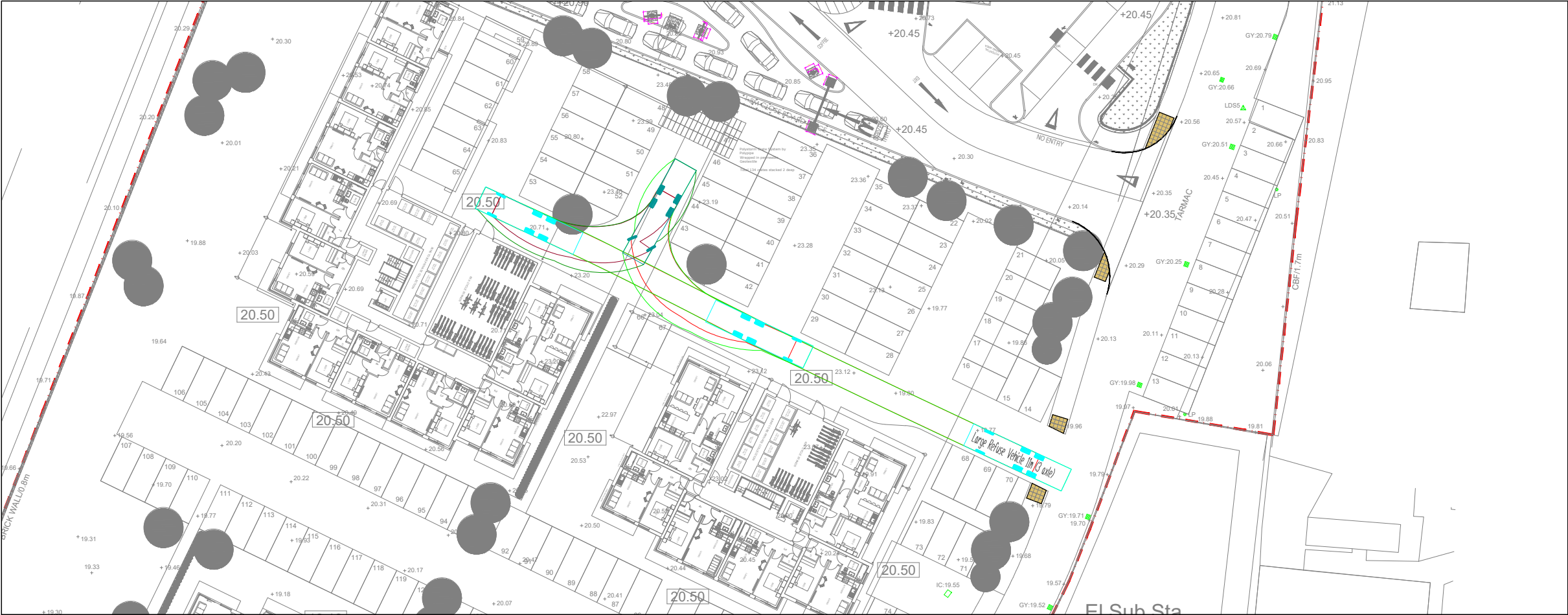
REFUSE VEHICLE TRACKING 1
