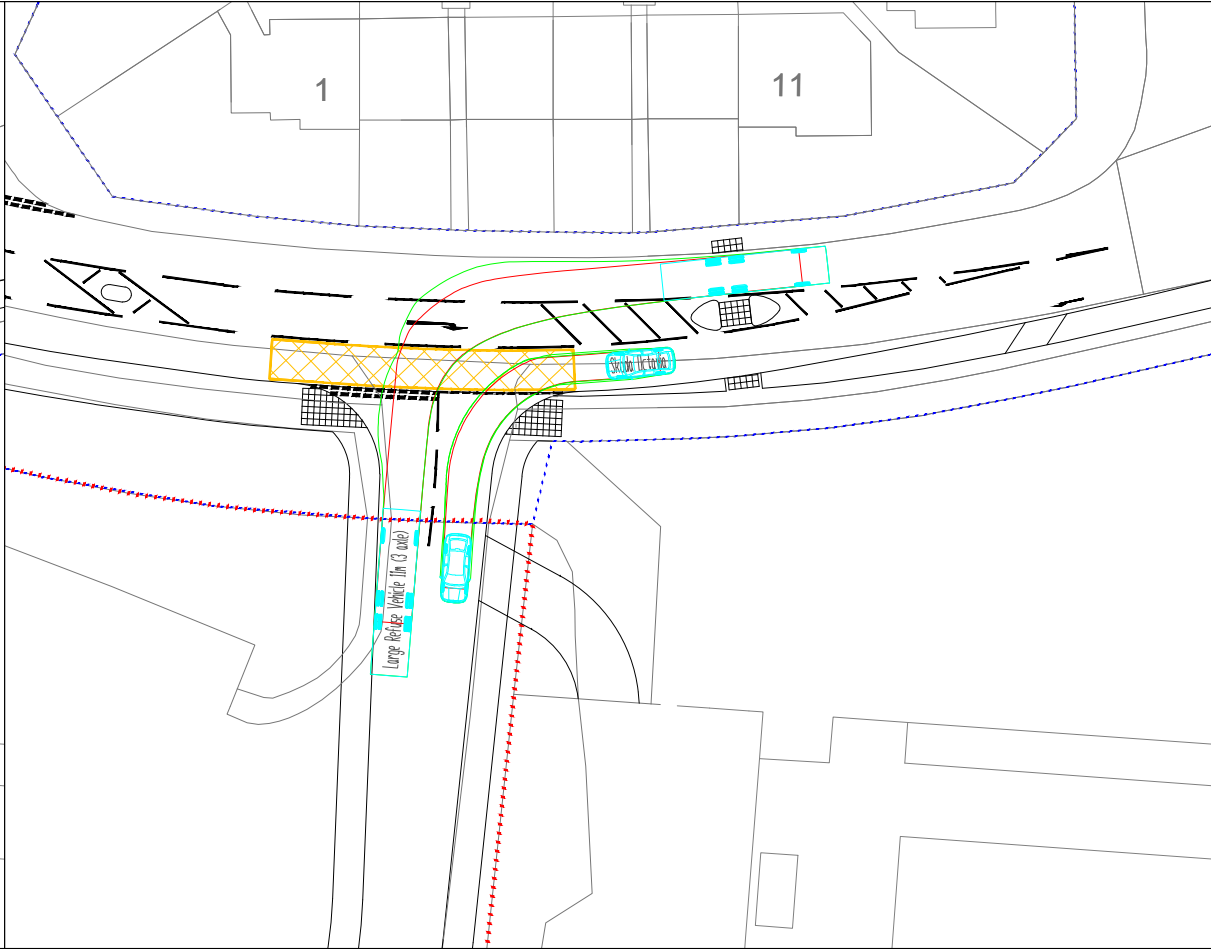
LARGE REFUSE VEHICLE – RIGHT OUT
