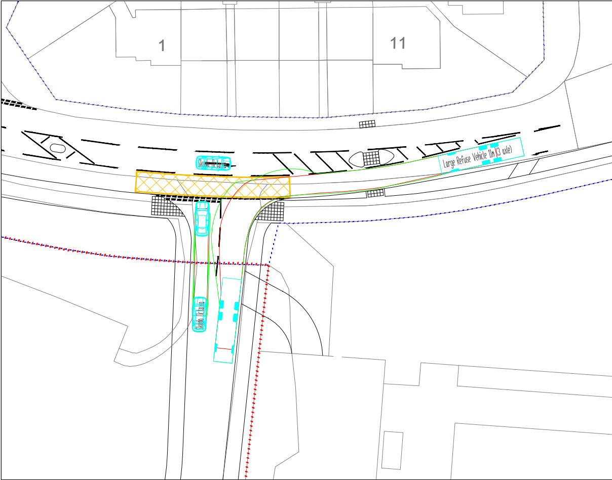
LARGE REFUSE VEHICLE – LEFT IN
