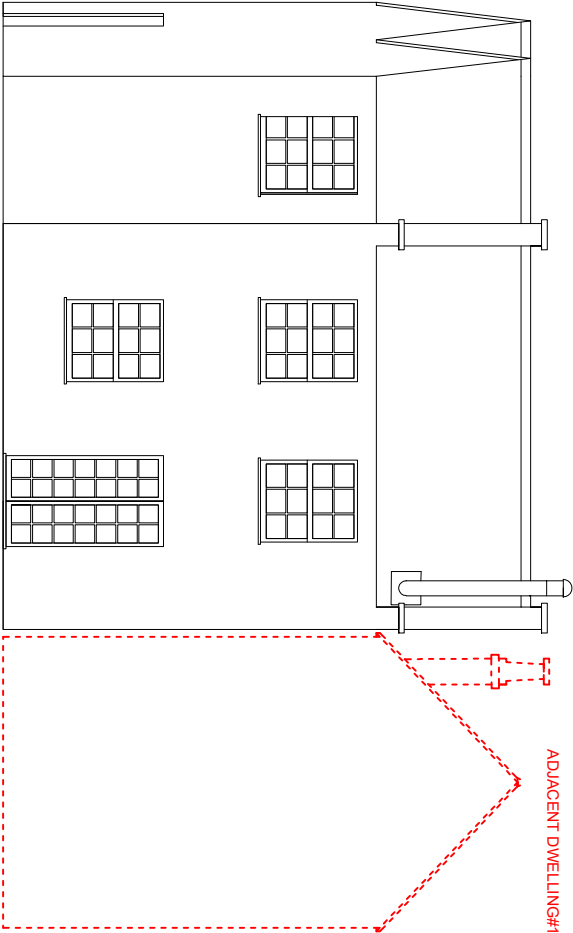
PROPOSED REAR (NW) ELEVATION
