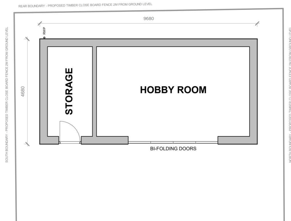
OUTBUILDING FLOOR PLAN 1 : 100
