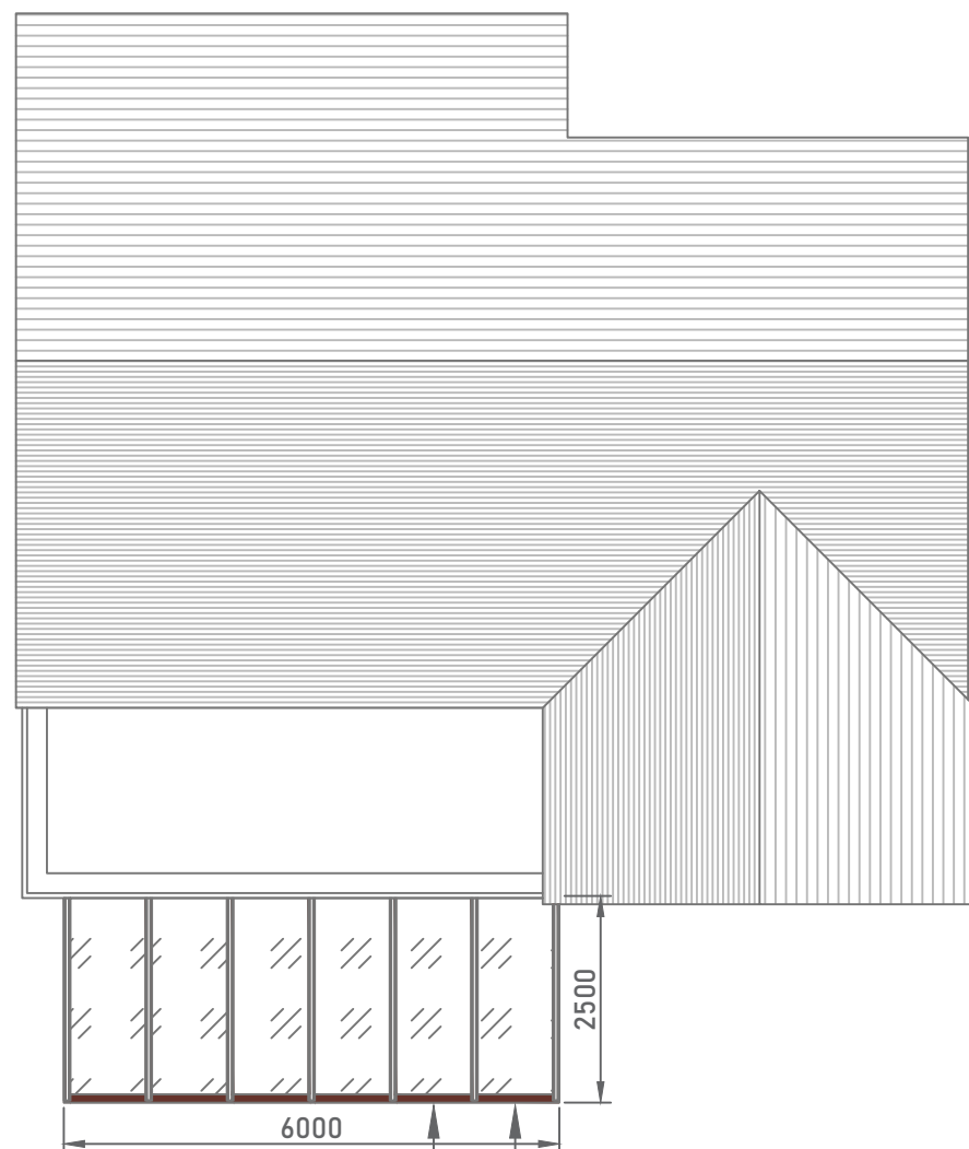
ROOF PLAN
