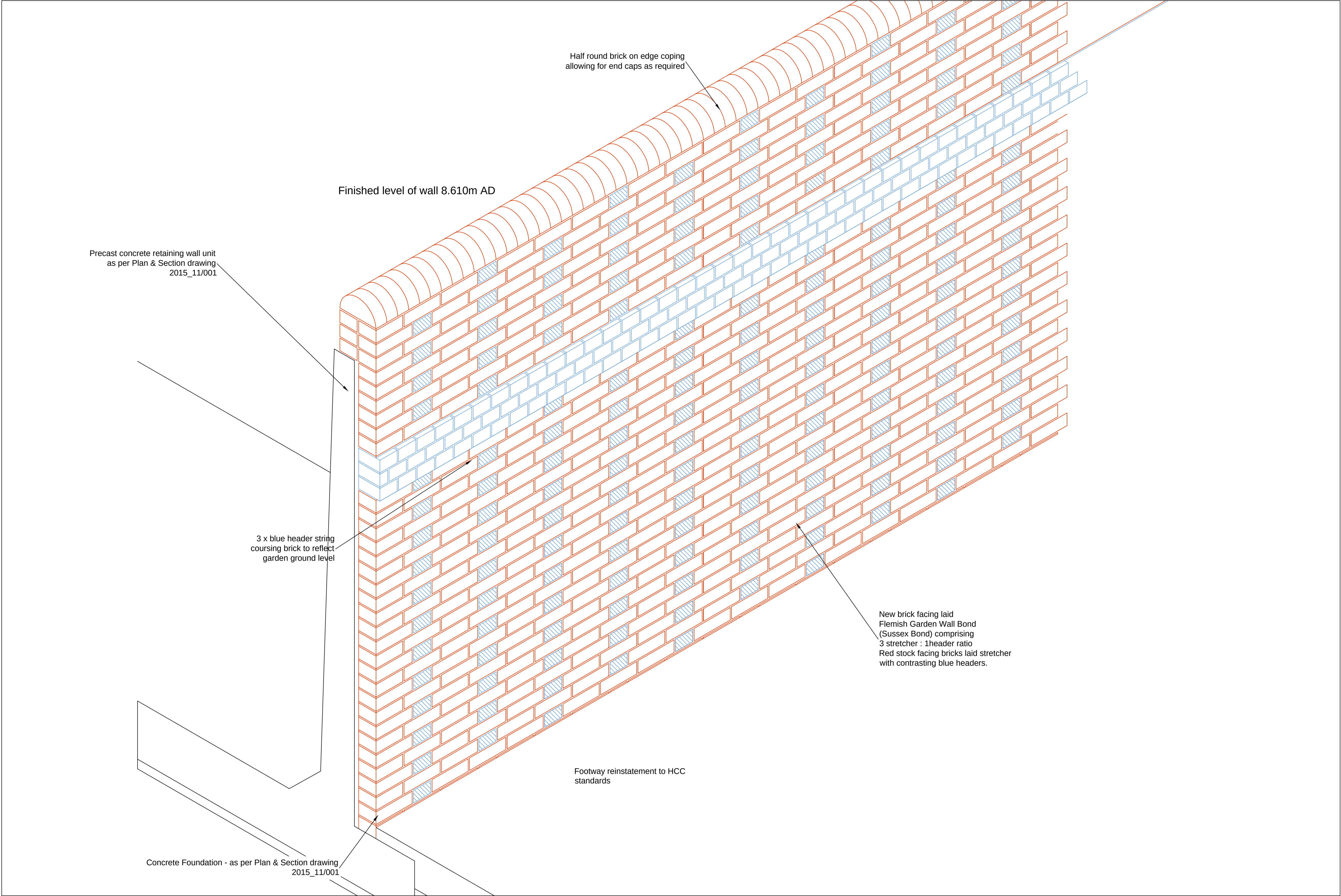
RETAINING WALL ISOMETRIC VIEW (APPROX. SCALE 1 : 10 BUT VARIES WITH PCC RETAINING UNIT TYPE)
