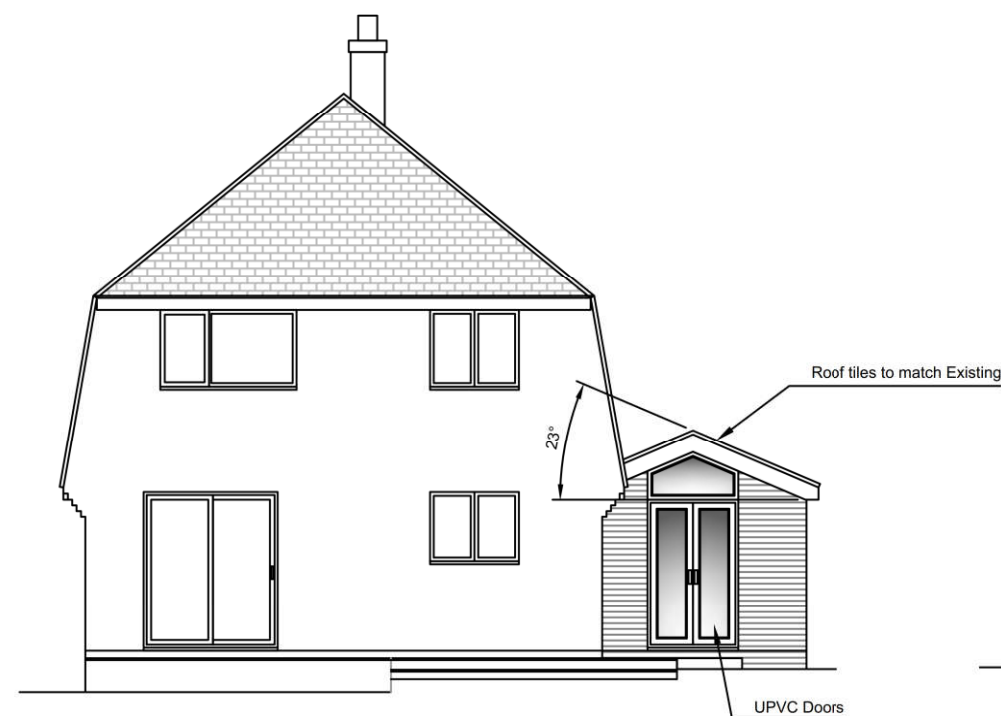
Rear Elevation
