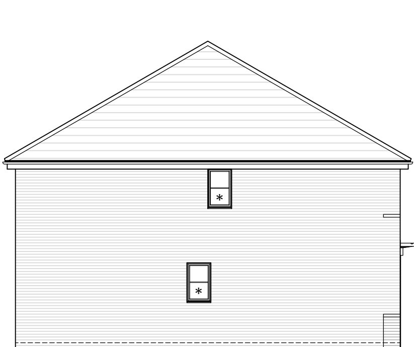
Side Elevation *No side windows to plots 69, 70, 154
