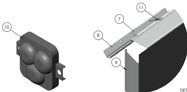
DETAIL B SCALE 1:1
