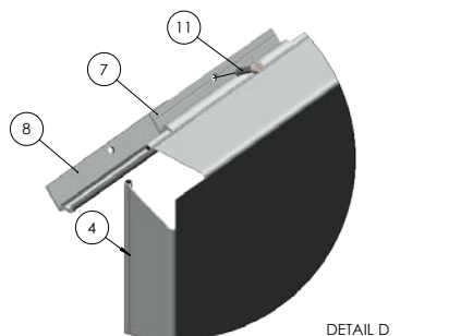
DETAIL D SHOWING SLIDING SPLIT CLAMP SCALE 1:2
