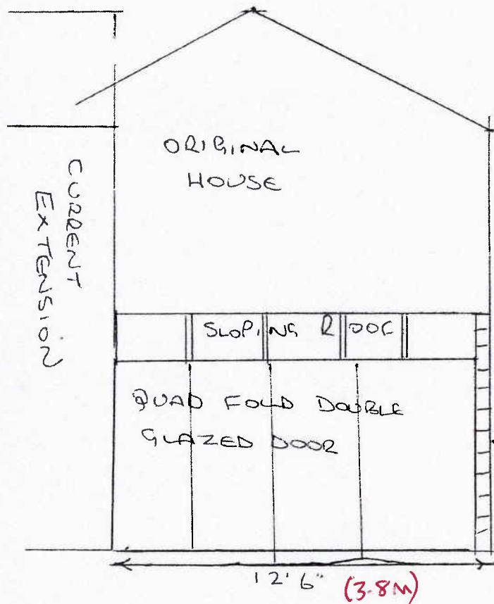
SIDE ELEVATION
