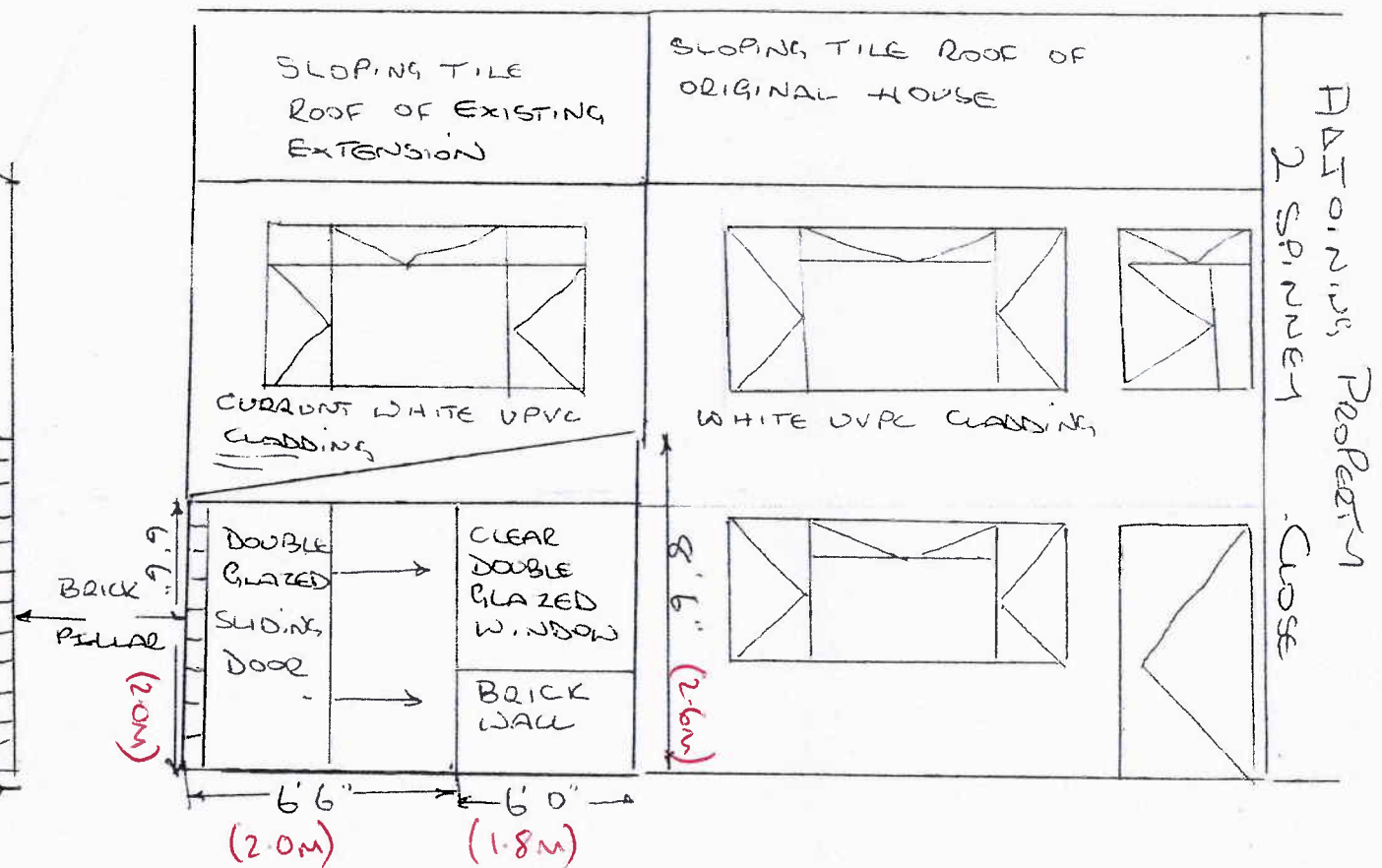
FRONT ELEVATION
