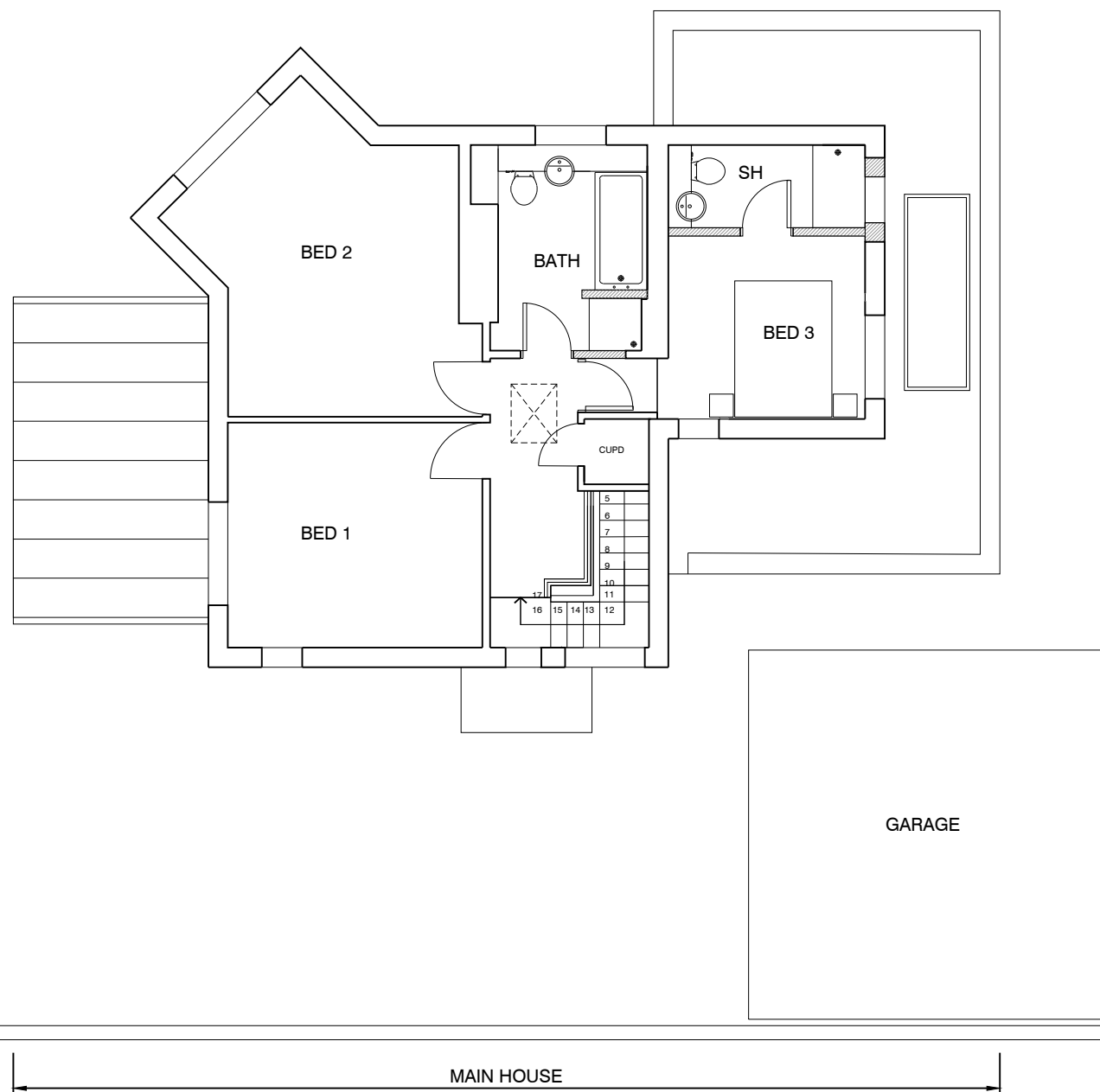
PROPOSED FIRST FLOOR PLAN - MAIN HOUSE SCALE 1:100 @ a3
