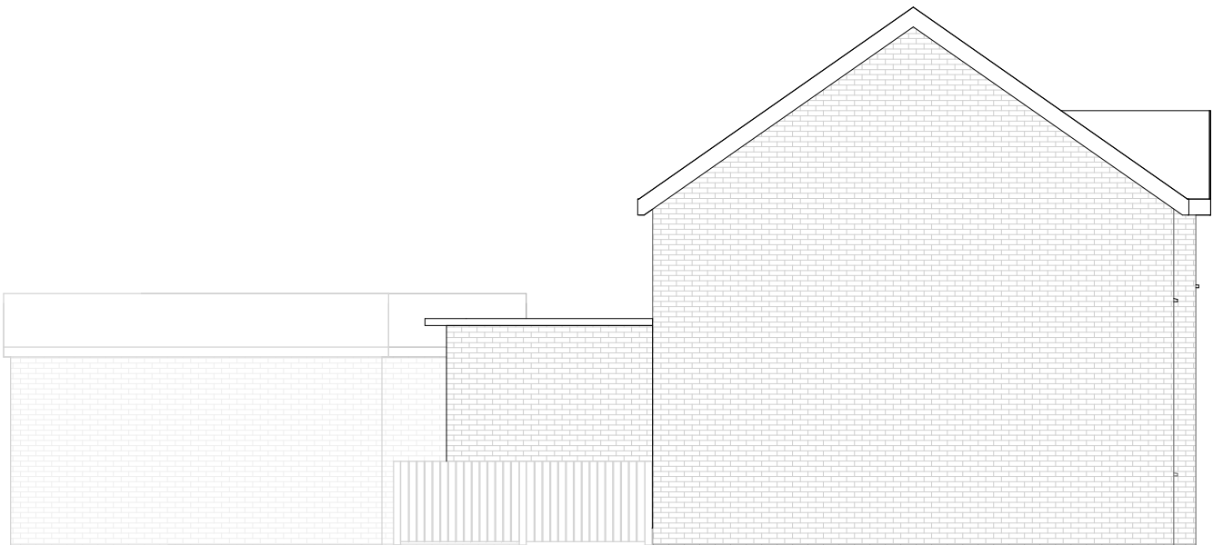
Proposed Elevation-Left side
