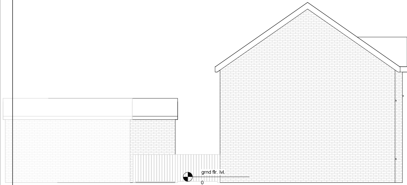
Existing Elevation-Left side
