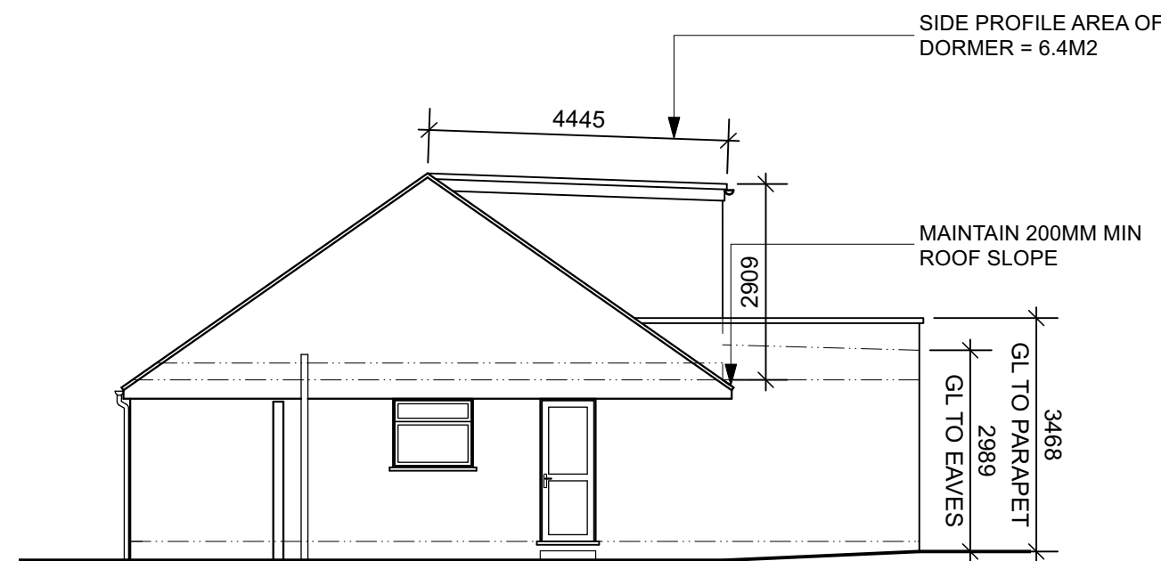
7 Proposed South Elevation Scale: 1:100
