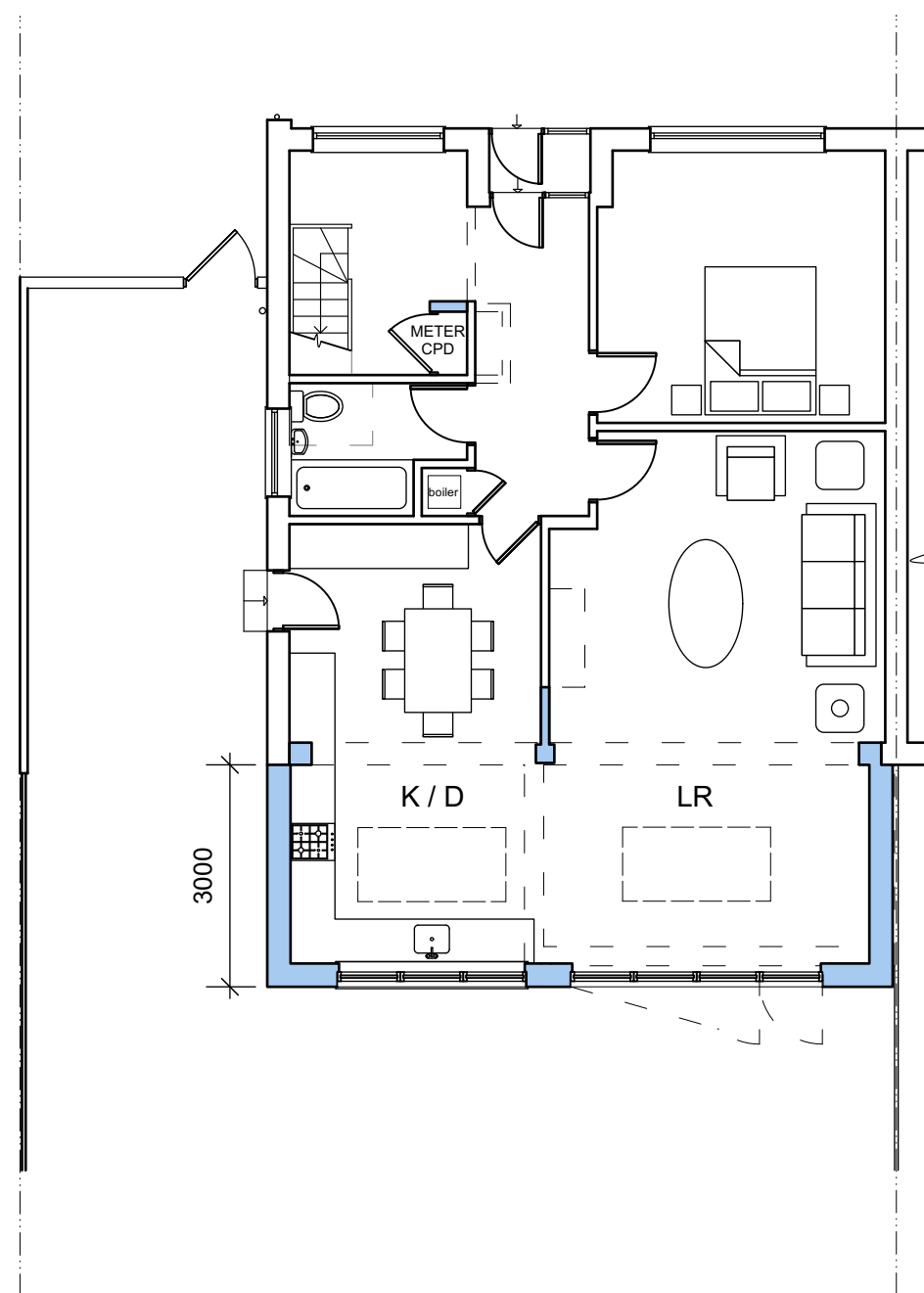
6 Proposed First Floor Plan Scale: 1:100
