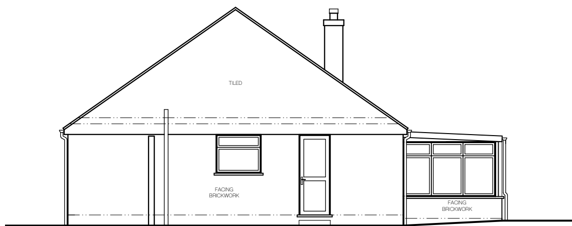
2 Existing South Elevation Scale: 1:100
