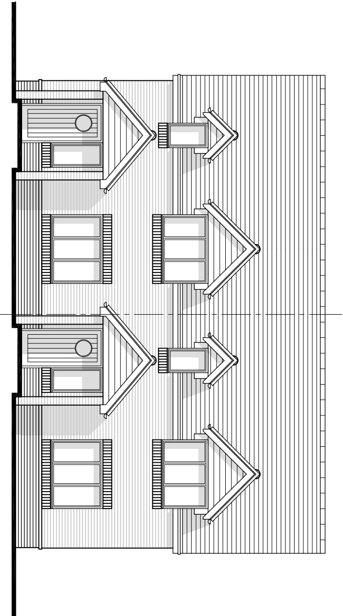
PLOT 9 SOUTH ELEVATION
