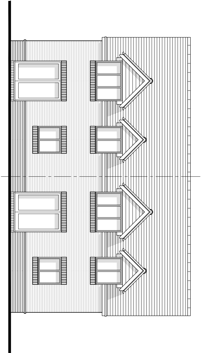
PLOT 10 NORTH ELEVATION
