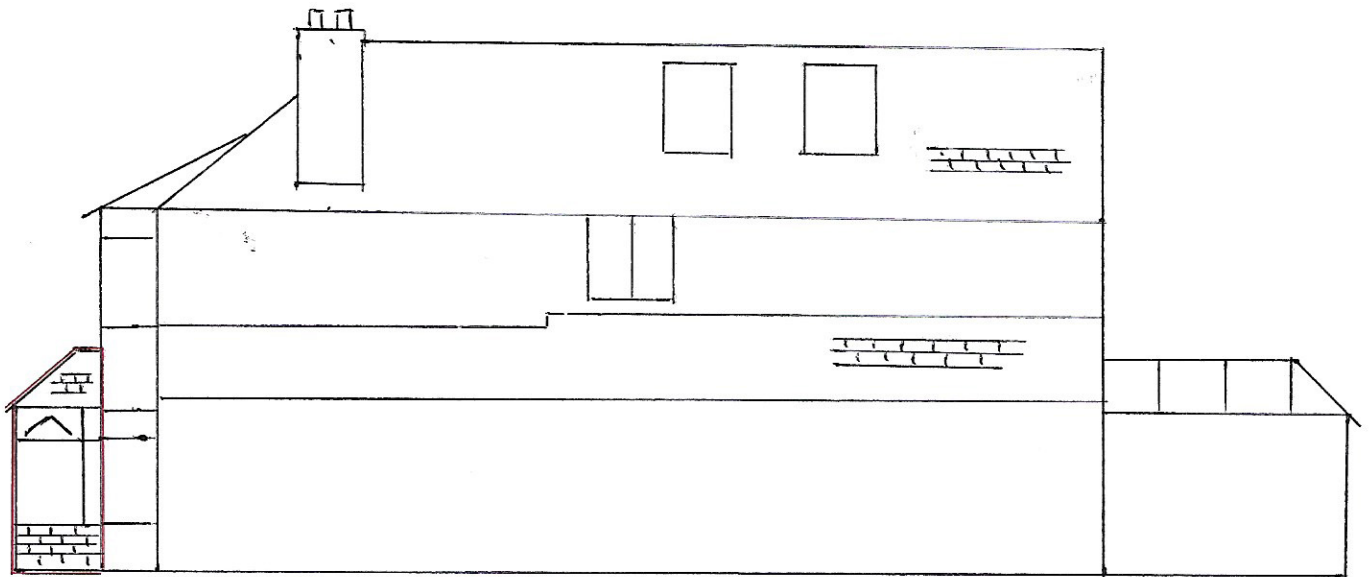
RH Side Elevation - Proposed
