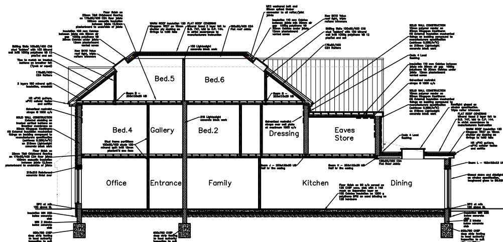
SECTION C-C
