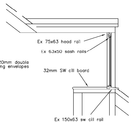
Dormer Section
