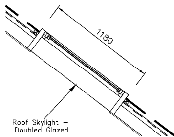
Velux M06 Section
