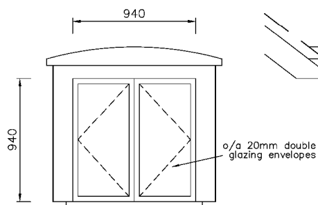
Dormer Elevation
