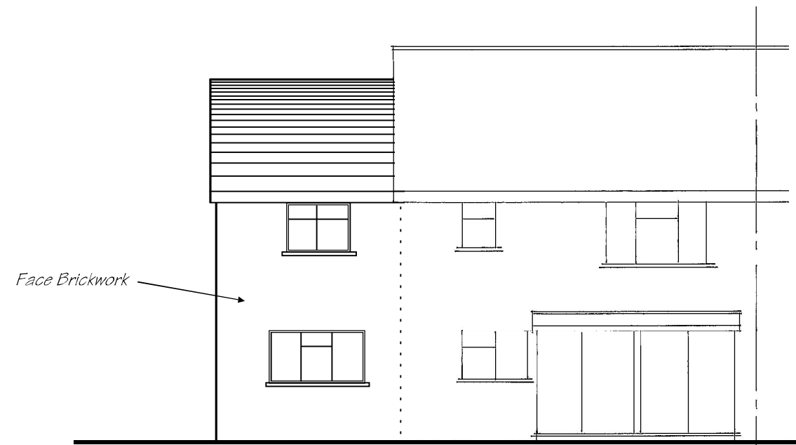
Proposed SE/Rear Elevation
