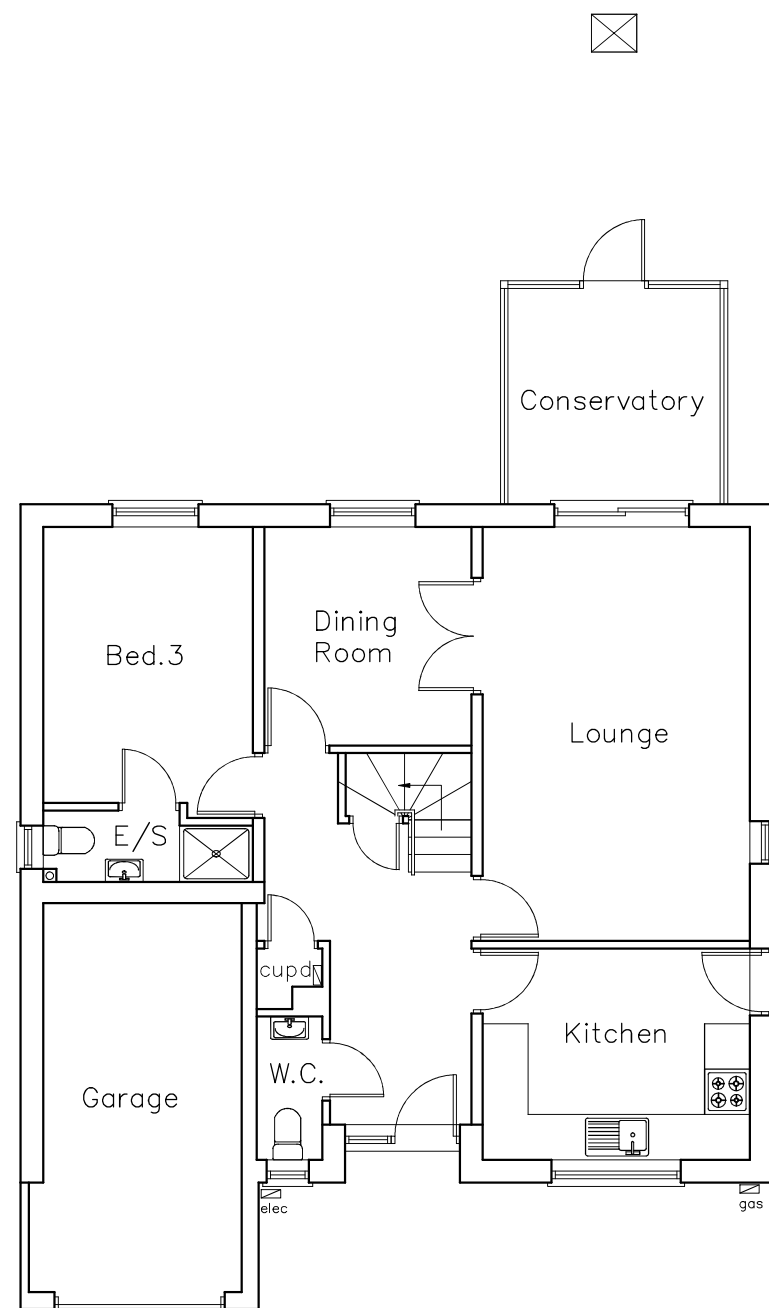
GROUND FLOOR
