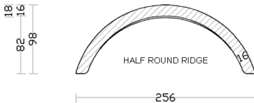
Redland half round ridge tiles
