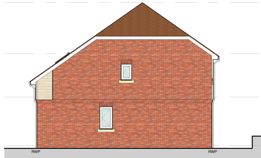
SIDE (SOUTH EAST) ELEVATION Scale 1:100
