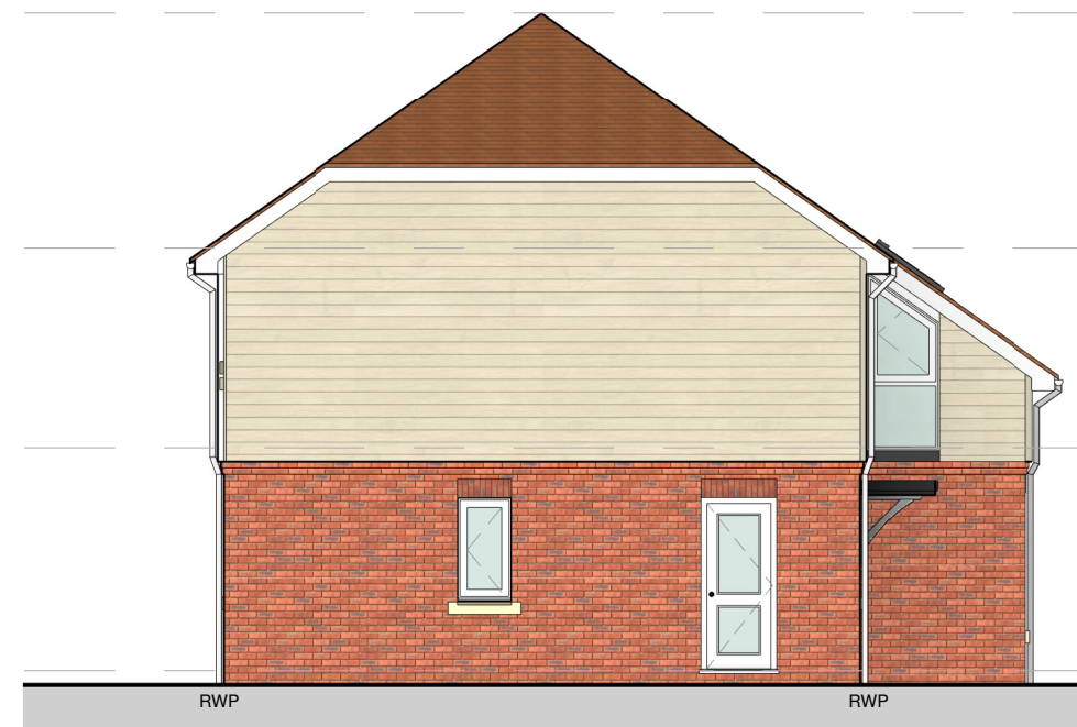
SIDE (NORTH WEST) ELEVATION Scale 1:100
