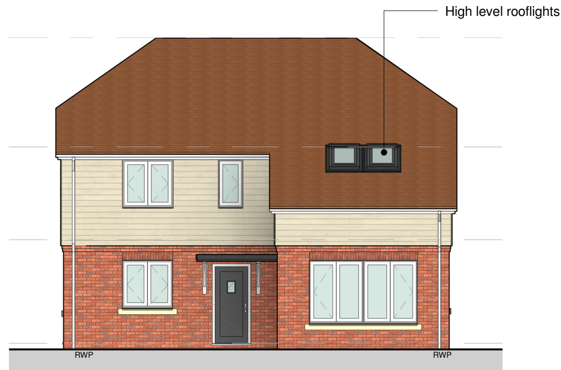
FRONT (SOUTH WEST) ELEVATION Scale 1:100
