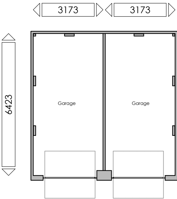
Floor Plan
