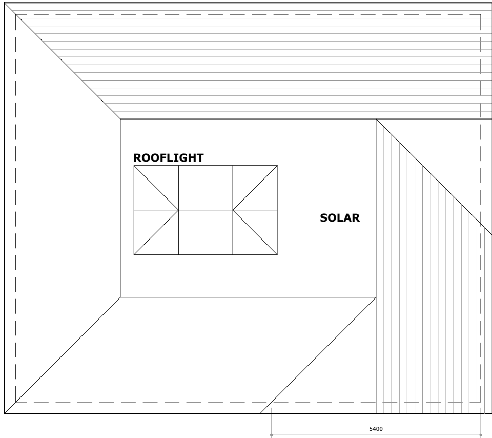
ROOF PLAN
