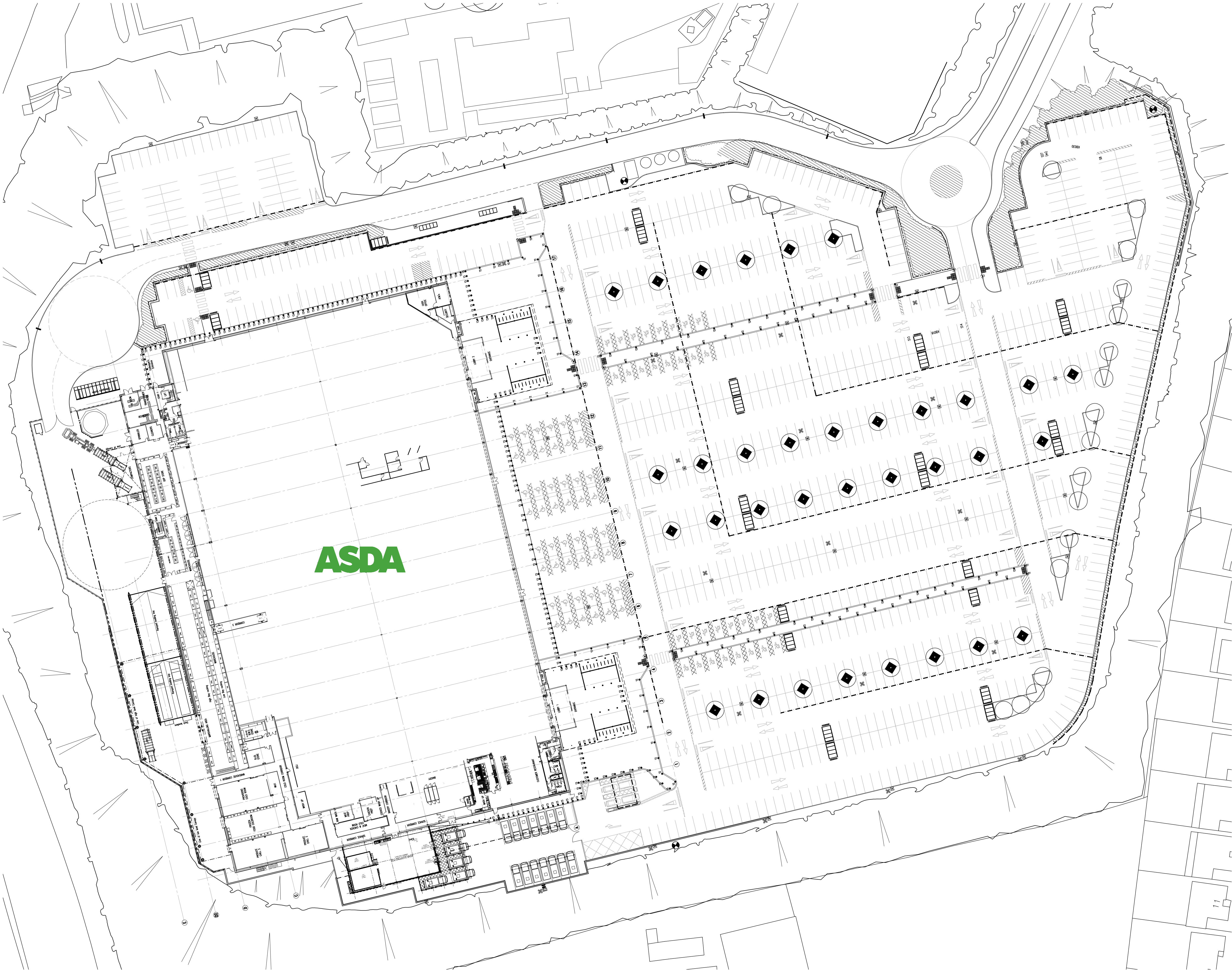
1 EXISTING SITE LAYOUT PLAN PL-02 Scale 1:500 @ A1
