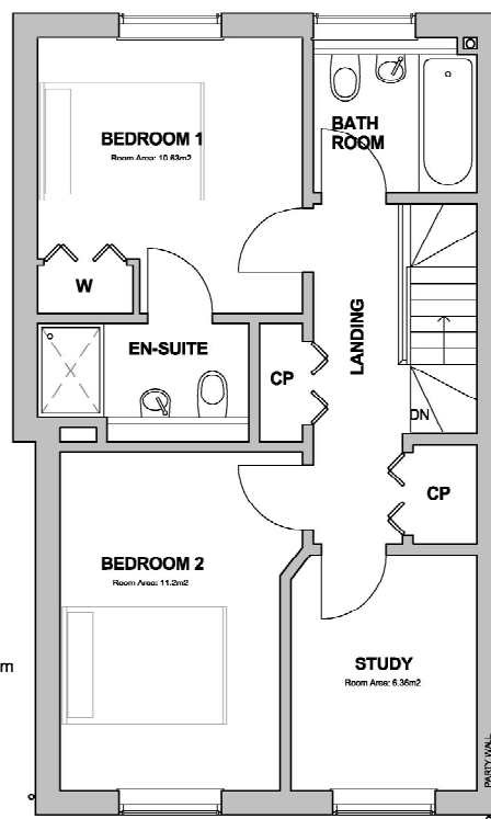
DWELLING 1 - FIRST FLOOR PLAN 1 : 50
