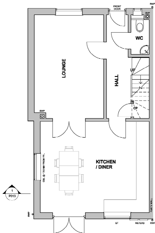
DWELLING 1 - GROUND FLOOR PLAN 1 : 50
