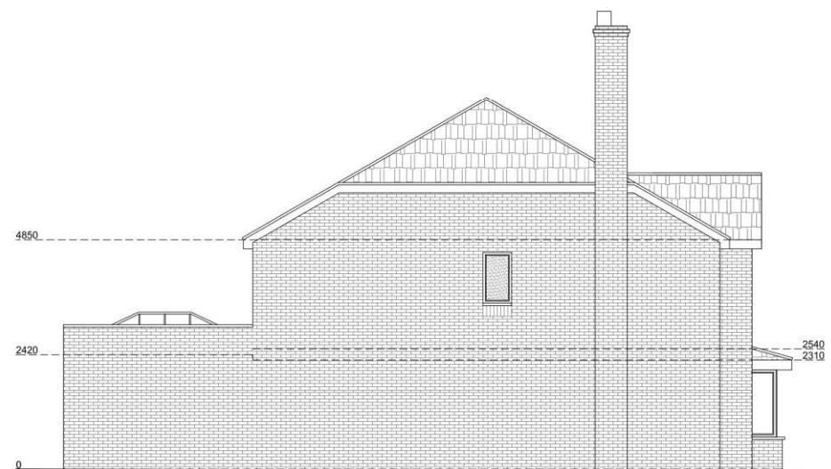
Existing West Elevation Scale 1:50
