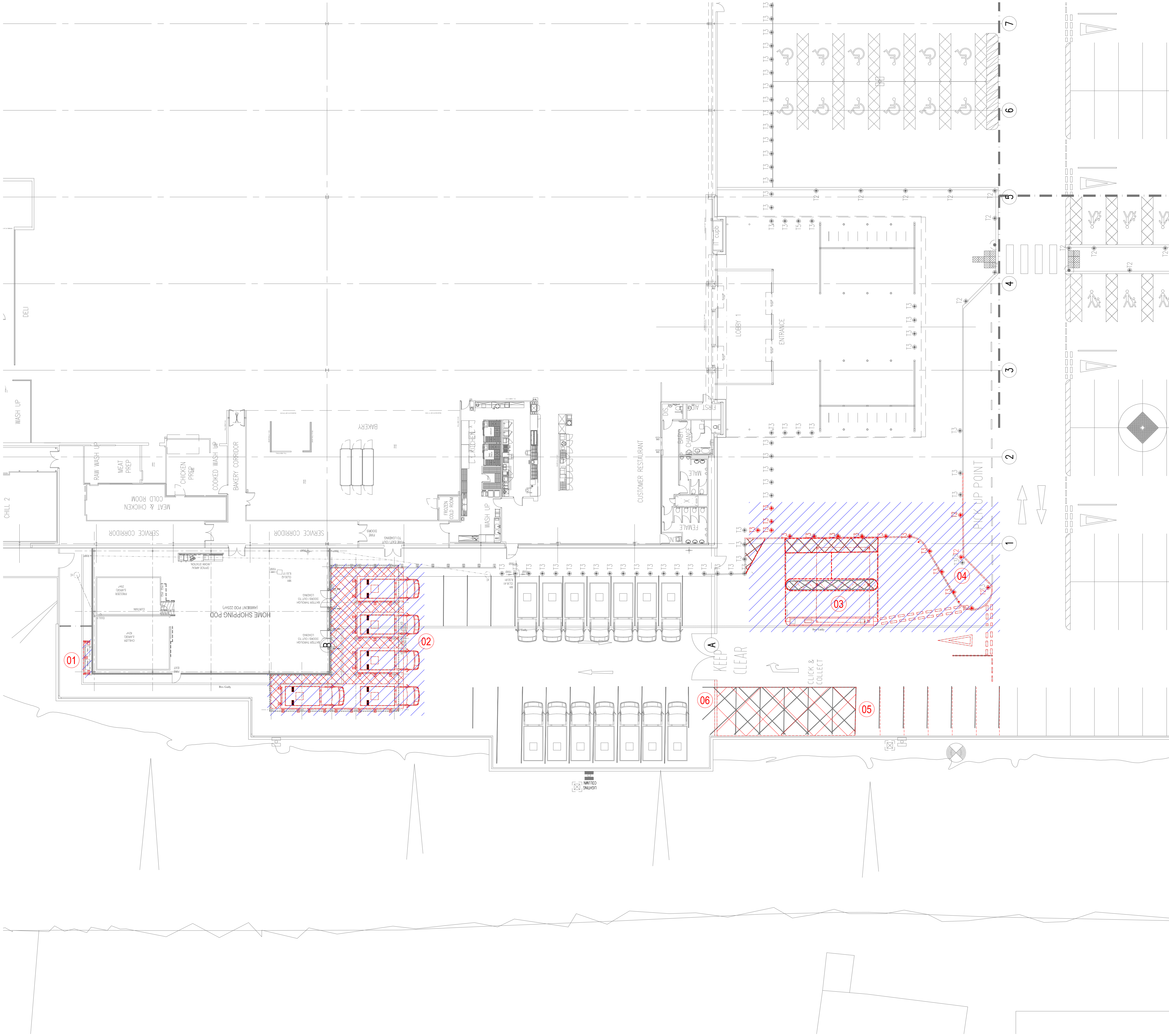
1 GROUND FLOOR DEMOLITIONS PLAN PL-13 Scale 1:200 @ A1
