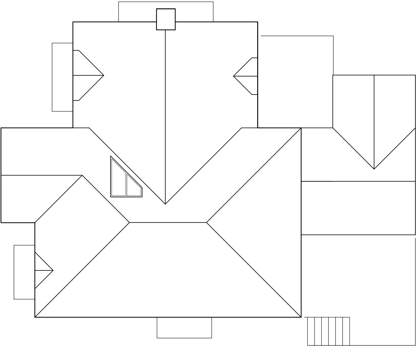
Roof 1:100
