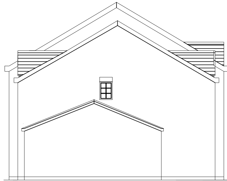
Proposed Elevation Side 1
