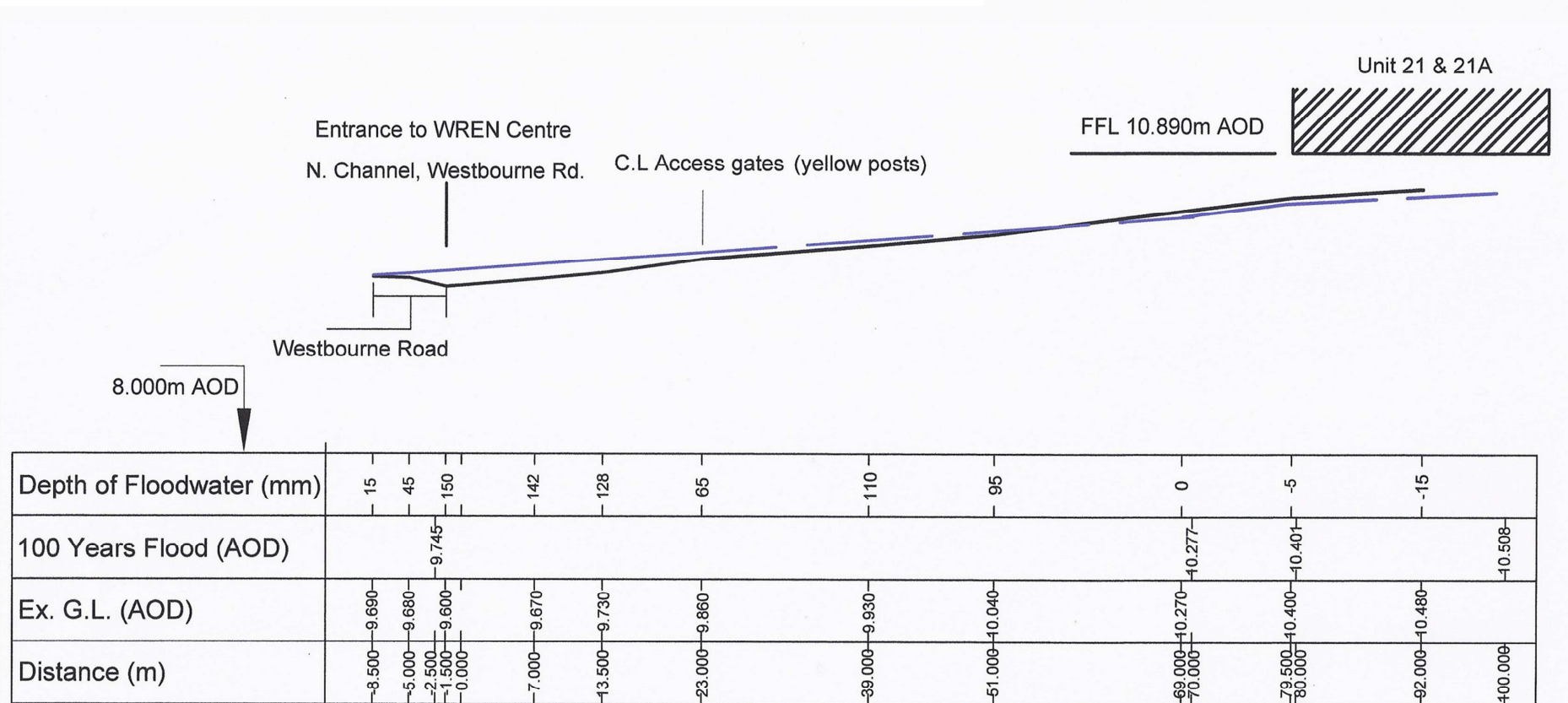
Section along Access Road B - B
