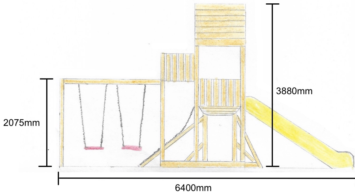
East side. View from 55a South Street (facing down the garden)
