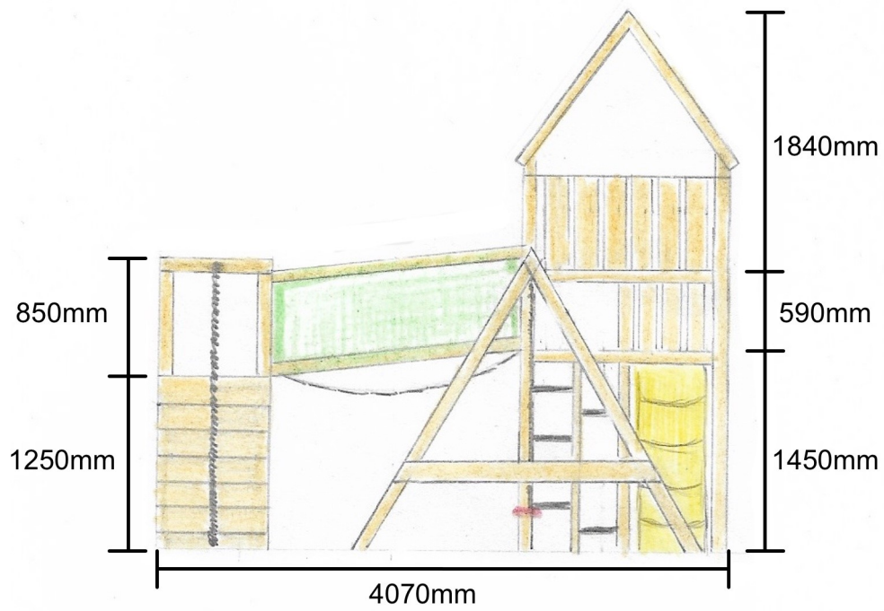
South side. View from 55 South Street
