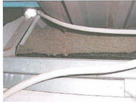
Rockwool behind external panels
