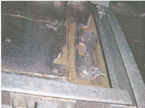
Foil encased Rockwool behind external panelling in roof plant room
