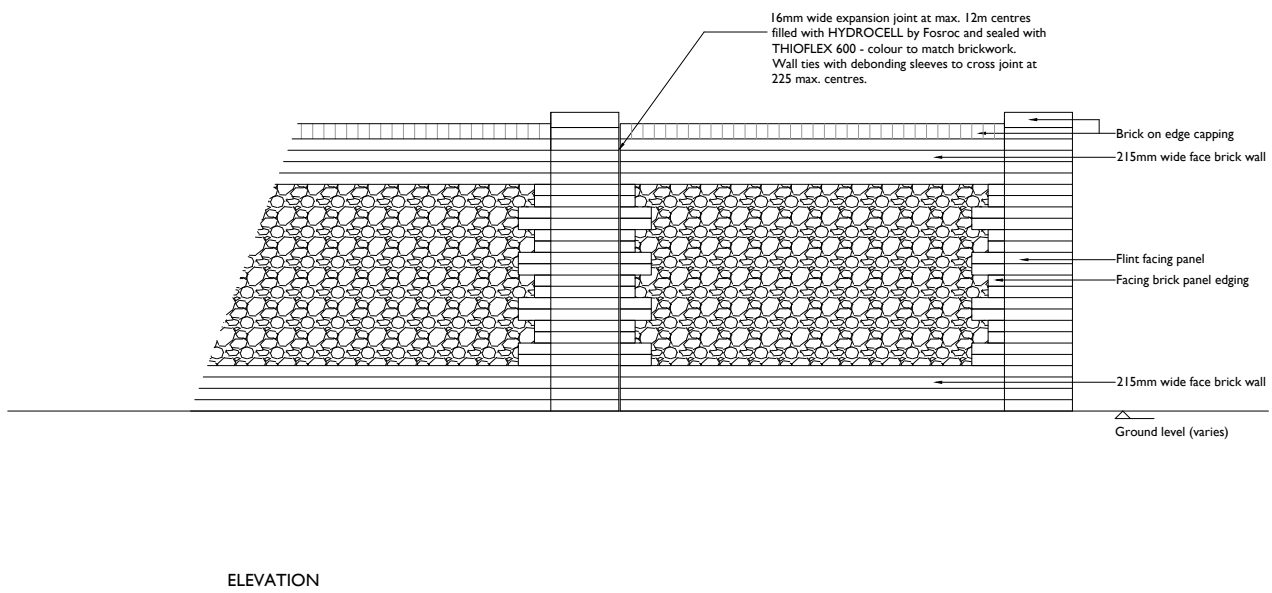
Typical Brick & Flint Panel Wall within development - 1800mm high
