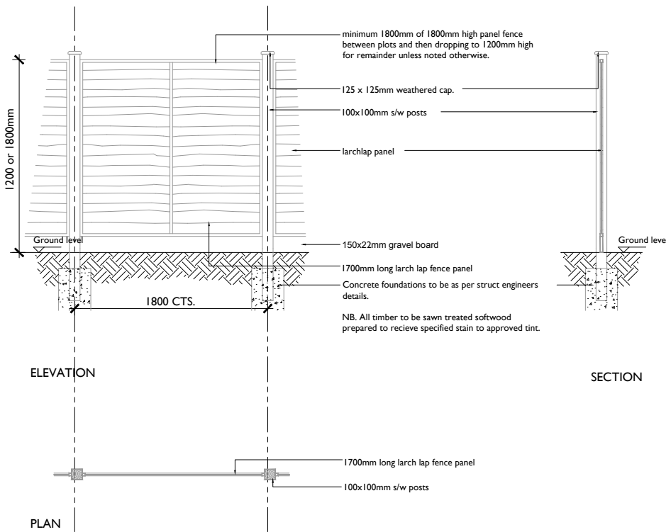
Typical Larch Lap Fence - 1200 or 1800mm high (Private garden area boundaries)
