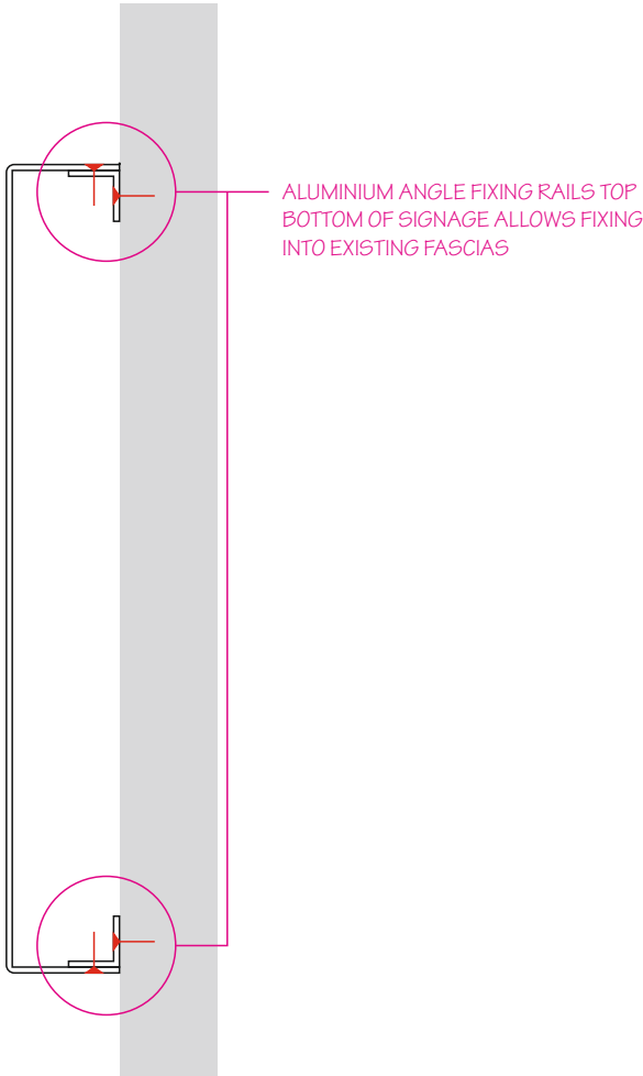
SIGNS 2 + 4 FIXING DETAIL
