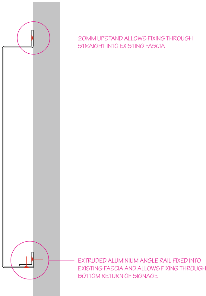
SIGN 1 FIXING DETAIL
