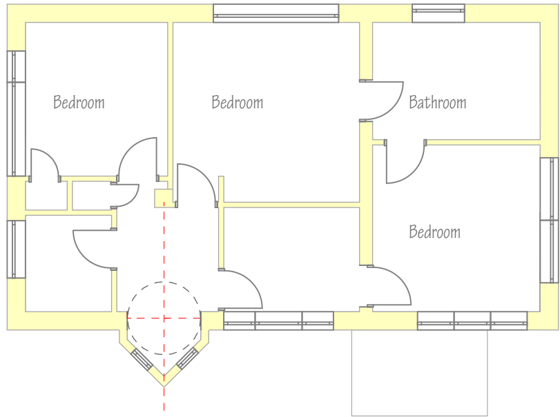
First Floor Plan as Existing @ 1:100
