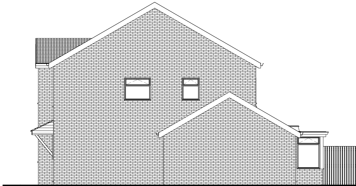
4 West Elevation 1 : 100
