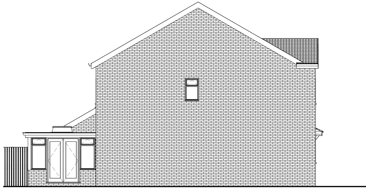
1 East Elevation 1 : 100
