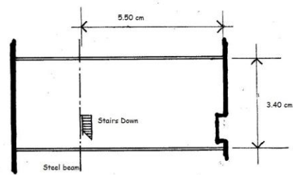
1:100 FLOOR PLAN
