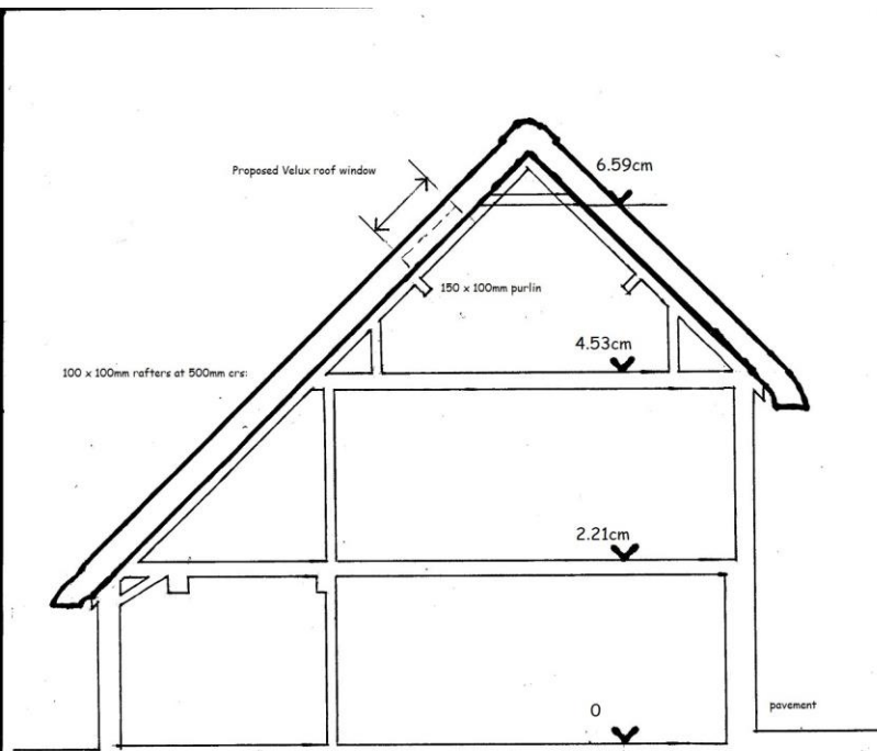
1:50 SECTION
